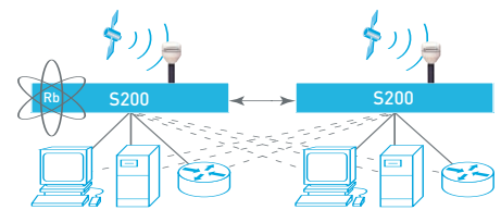
Redundant, resilient and secure configuration incorporating a Rubidium Oscillator in the primary server and peering to another primary server for backup redundancy.
