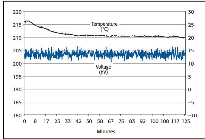
Figure 5. The Model 2182A's delta mode provides extremely stable results, even in the presence of large ambient temperature changes. In this challenging example, the 200nV signal results from a 20µA current sourced by a model 6221 through a 10mΩ test resistor.
