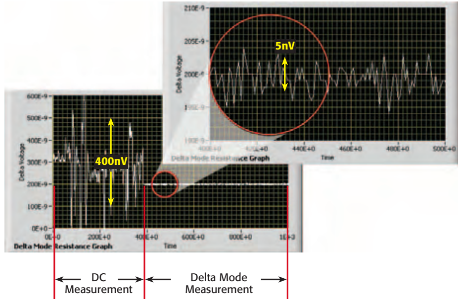
Figure 2. Results from a Model 2182A/6220 using the delta mode to measure a 10mΩ resistor with a 20µA test current. The free Model 6220/6221 instrument control start-up software used can be downloaded from www.keithley.com .
