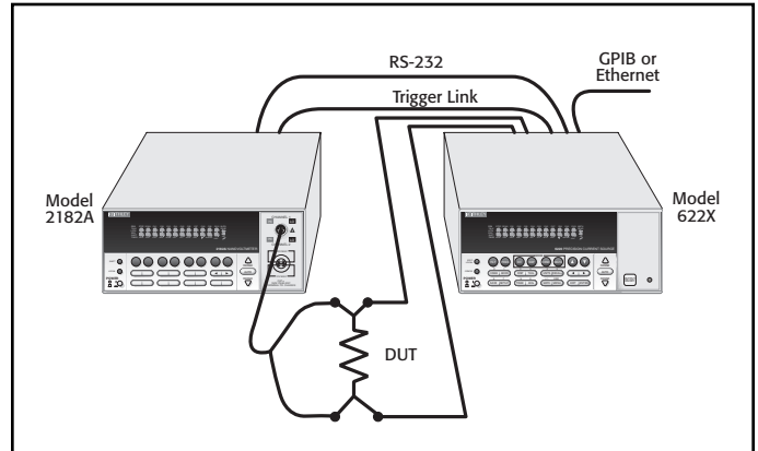
Figure 3. It's simple to connect the Model 2182A to the Model 6220 or 6221 to make a variety of measurements. The instrument control start-up software provided for the Model 622X current sources includes a step-by-step guide to setting up the instrumentation and making proper connections.
