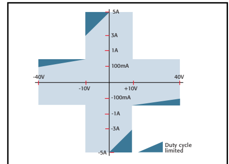
Model 2440 5A SourceMeter
