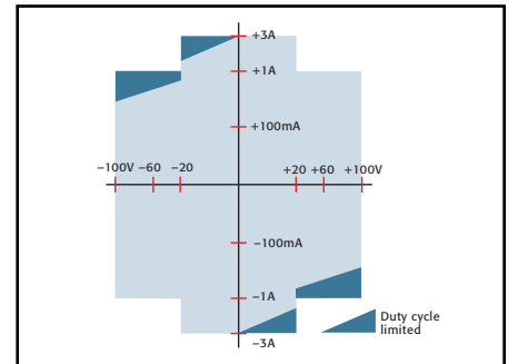
Model 2425 100W SourceMeter
