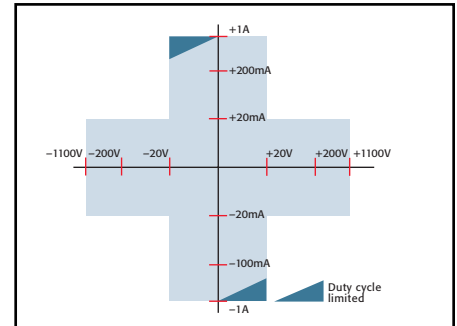
Model 2410 High-Voltage SourceMeter
