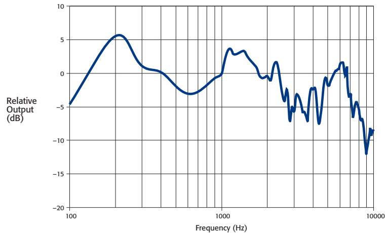
Figure 4. Frequency Response
